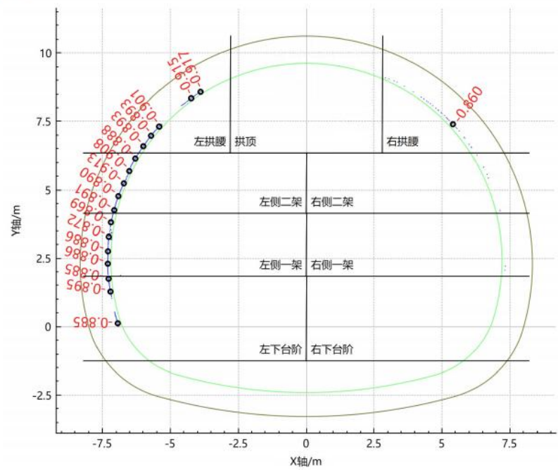
断面图:DK45+201.0
